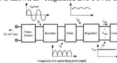
Fig:2. Block Diagram of Power Supply
