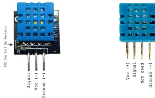
Figure.3.1 Front view of DHT11 sensor
